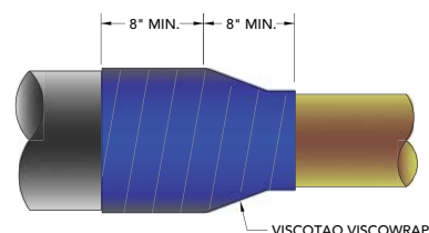
Fig. 4: Wrap ViscoWrap from casing pipe to carrier pipe. Start wrapping min. 8" from casing end and continue \geq 8" onto carrier pipe.
