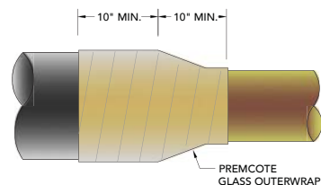
Fig. 5: Apply Premcote Glass Outerwrap over ViscoWrap layer. Start wrapping min. 10" from casing end and continue \geq 10" on carrier pipe.
