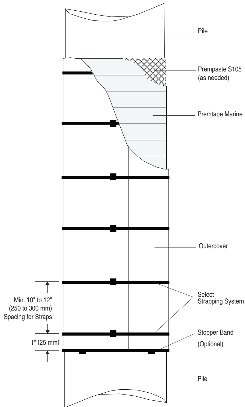
Elevation View
