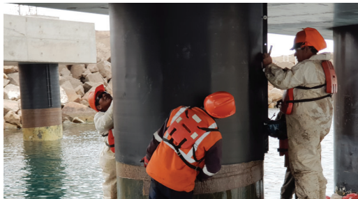
Contractor applying HDPE jackets in pile's upper part.
